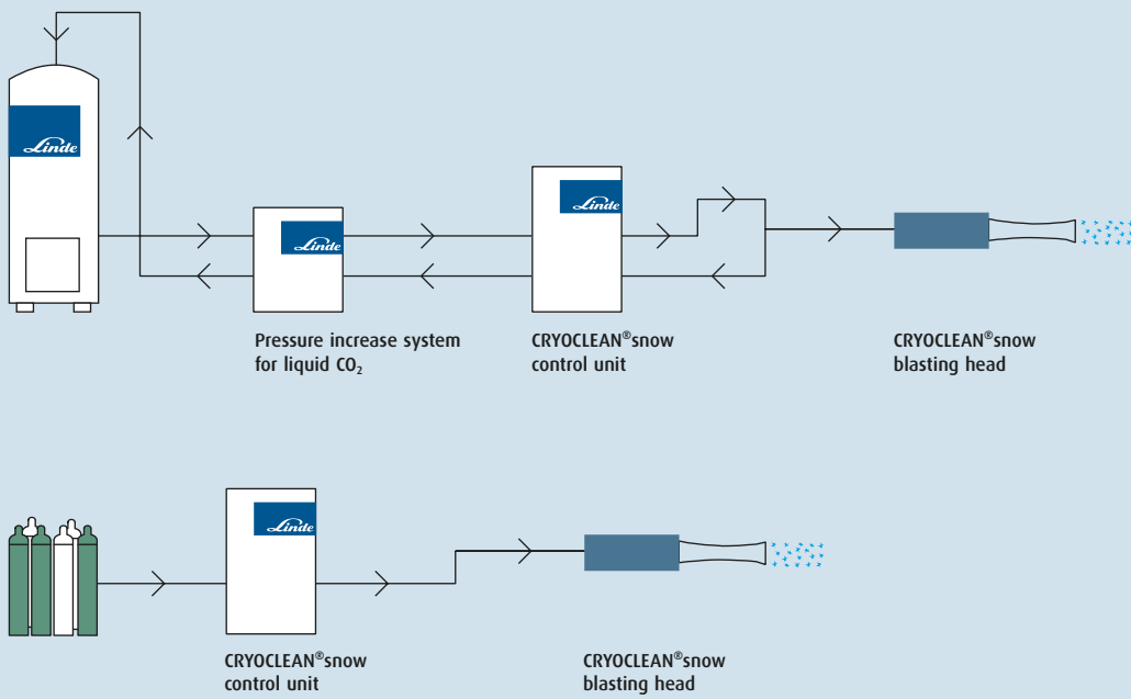
System assembly CRYOCLEAN®snow
