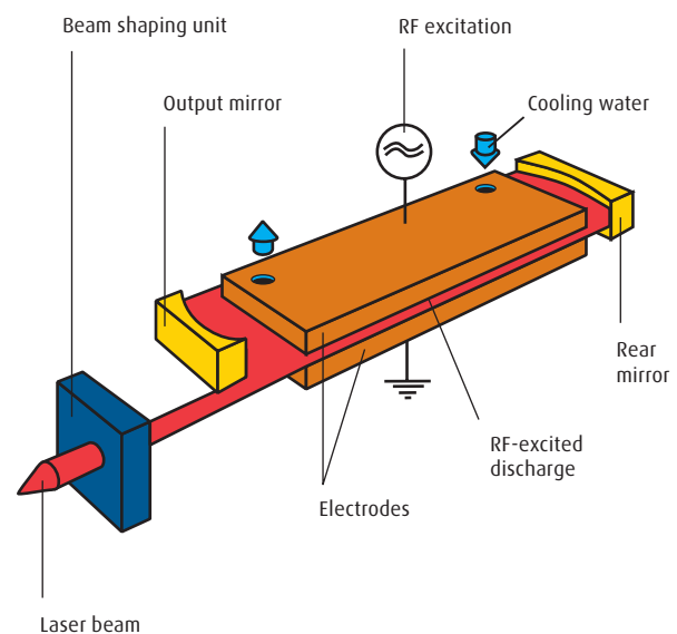
Fig. 11: Diffusion-cooled CO 2 laser
